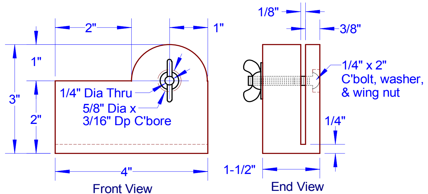
Plane Iron Holder
