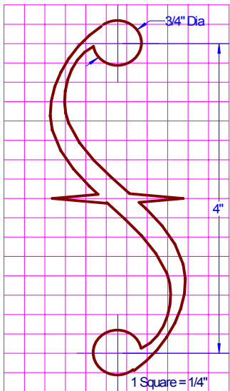
F-Hole Pattern
