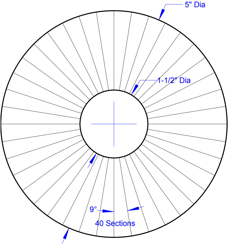
Indexing Disks
