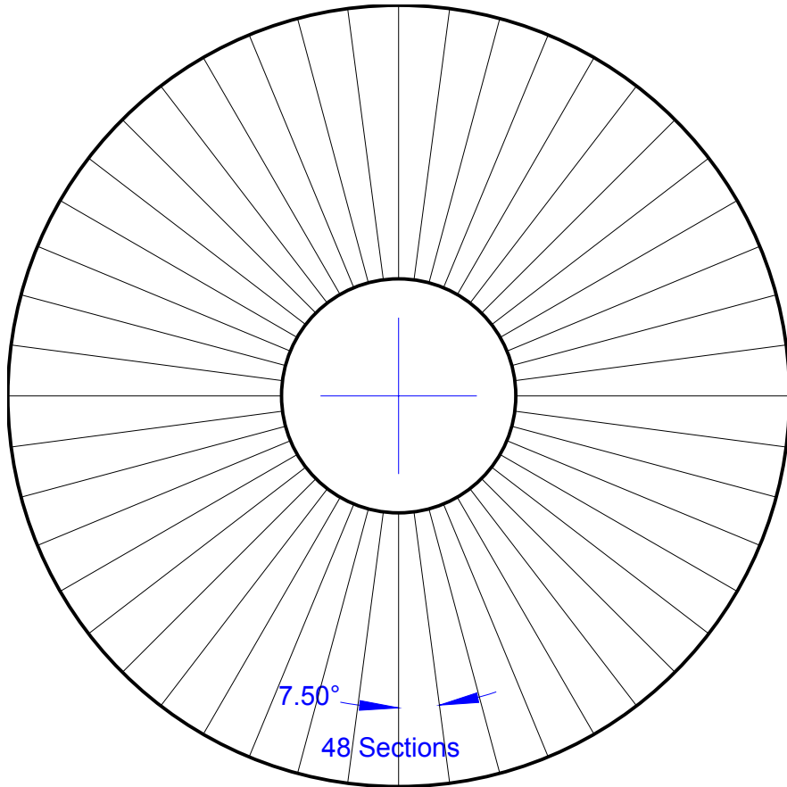
Indexing Disks
